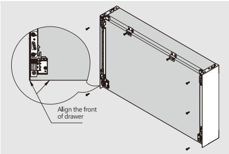
Align drawer sides and bottom, fix screws and fixing-brackets
