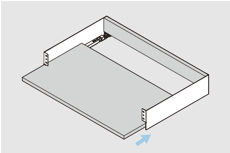
Bottom assembly
