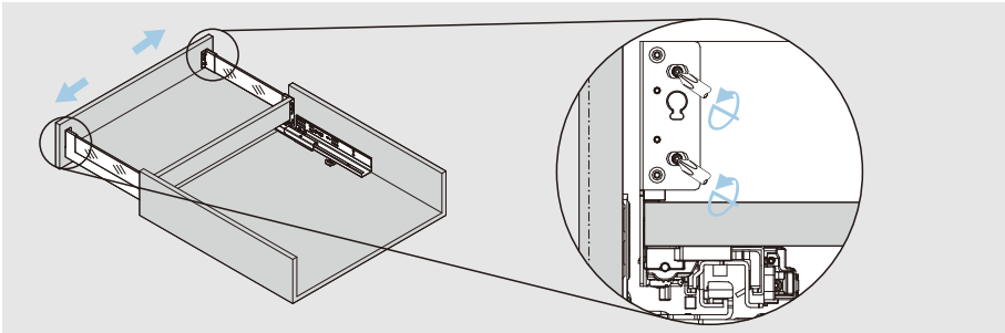
Left & right adjustment
