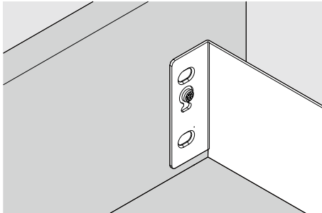
Insert the positioning pins into the key hole
