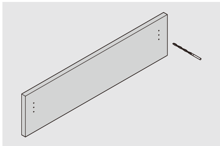
Pre-drill holes on the drawer front
