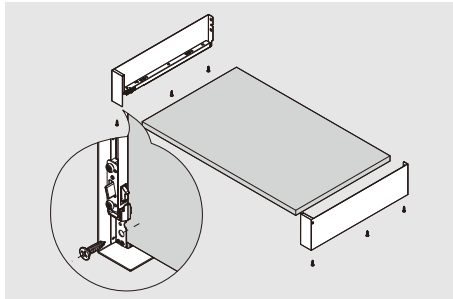
Align drawer sides and bottom, fix screws
