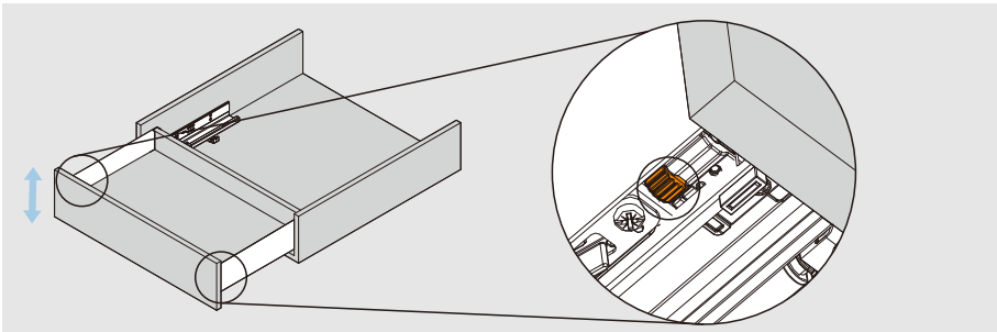
Up & down adjustment
