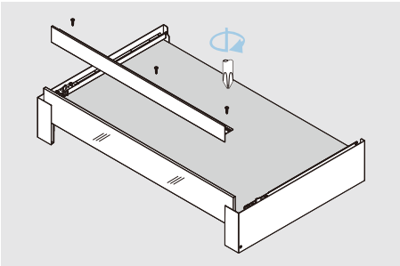
Install front section and front panel
