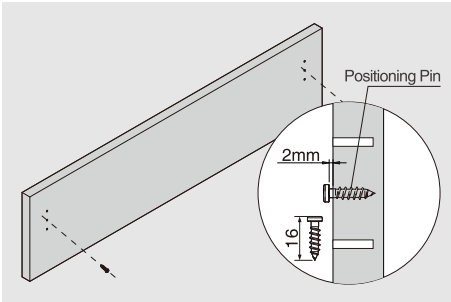
Install positioning pins
